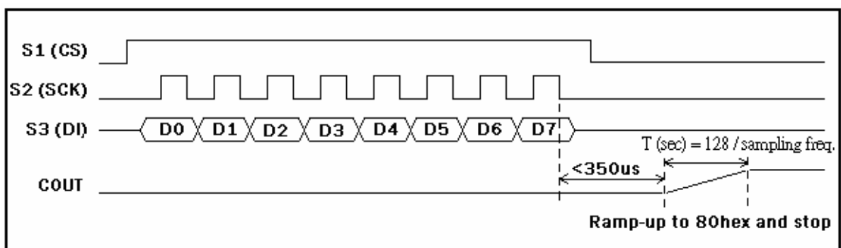
Fig. 11 Power-up command timing
