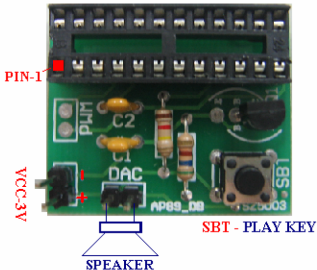
Part No. : AP89XS-DBD
