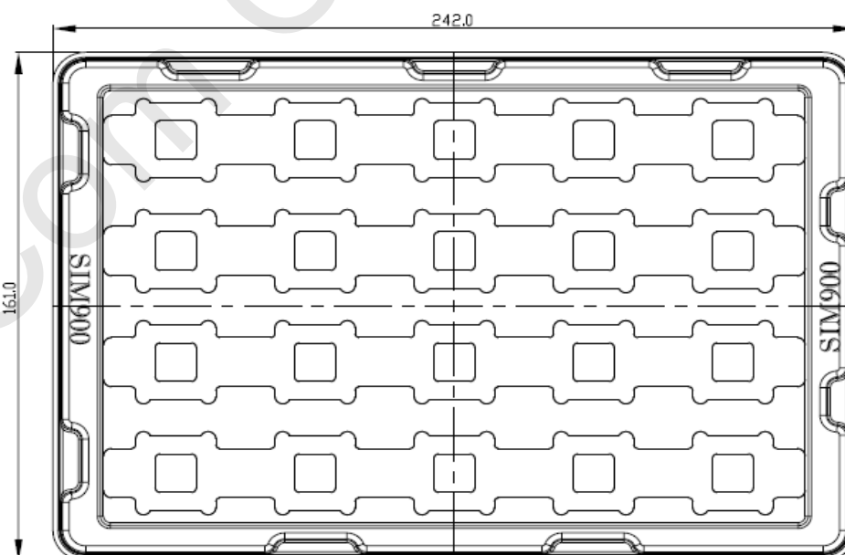
Figure 37: Tray drawing
