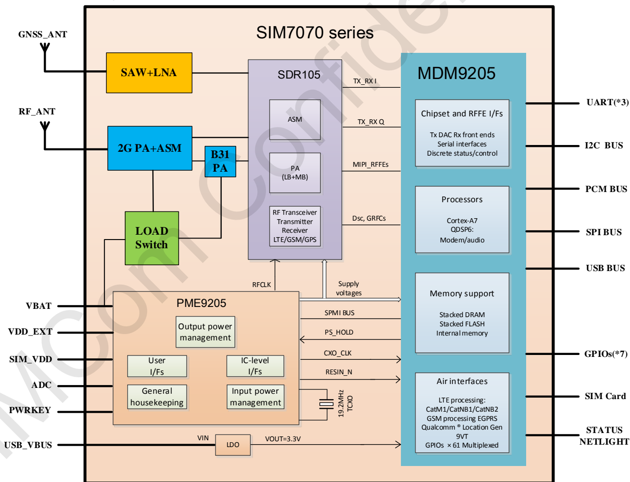
Figure 1: SIM7070 Series block diagram
