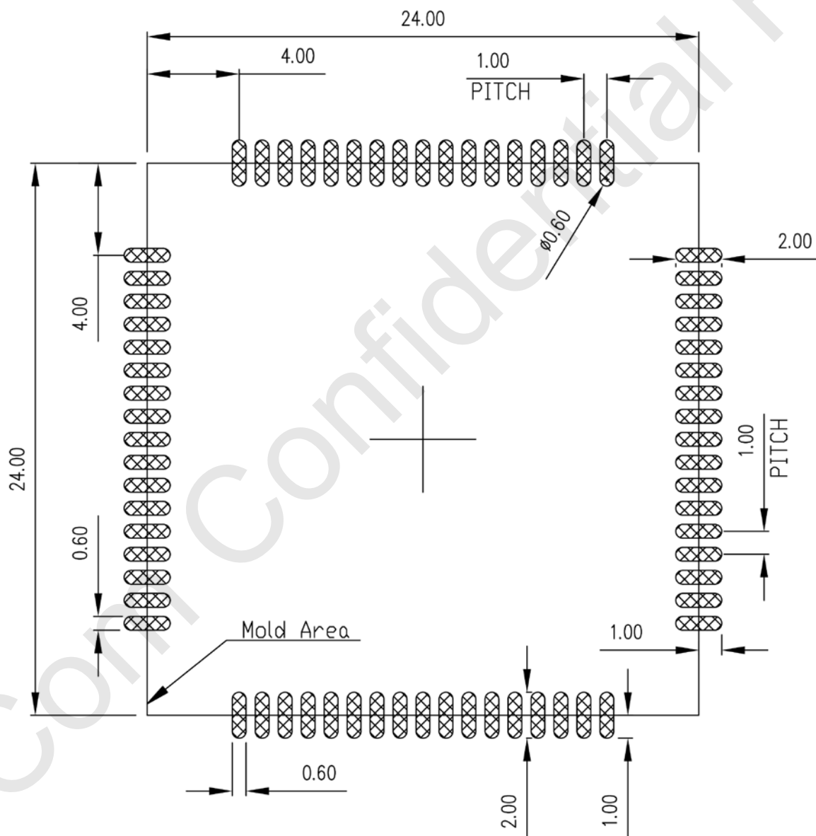
Figure 35: stencil recommendation (Unit: mm)
