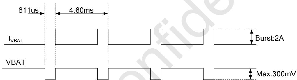
Figure 5: Voltage drop in EDGE or GPRS mode
