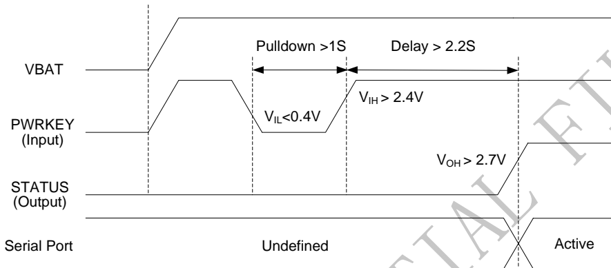
Figure 11: Timing of power on module
