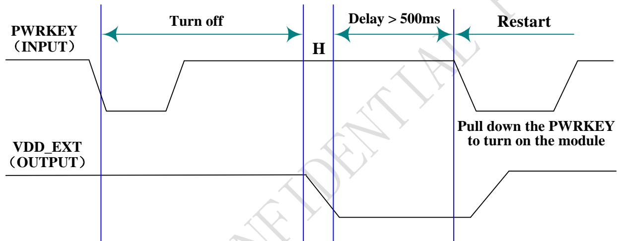
Figure 10: Timing of restart system
