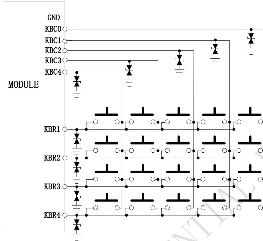
Figure 28: Reference circuit of the keypad interface
