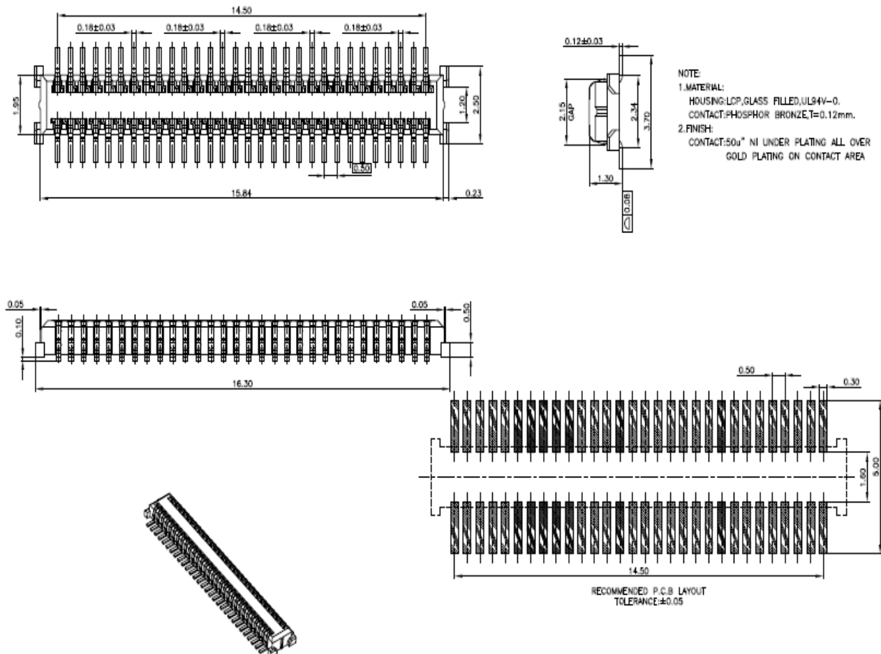
Figure 36: SUNCAGEY BB530-06001-20R board-to-board connector
