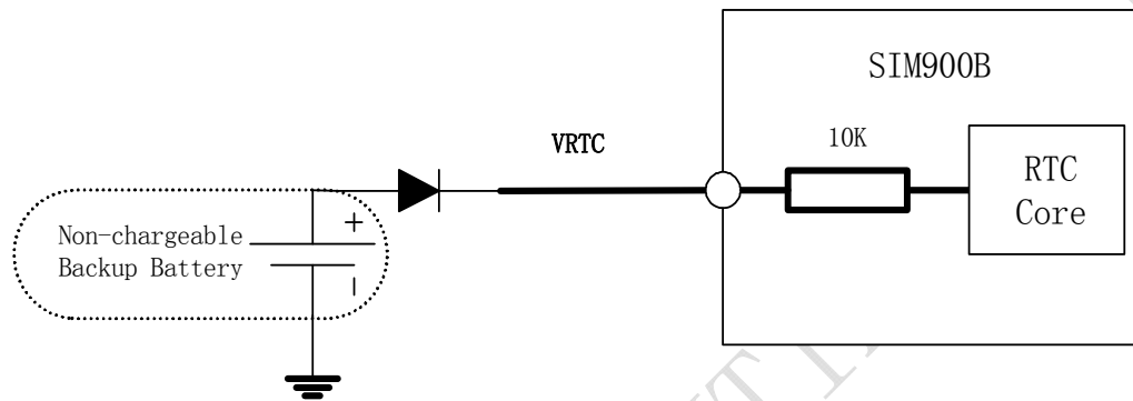
Figure 12: RTC supply from non-chargeable battery
