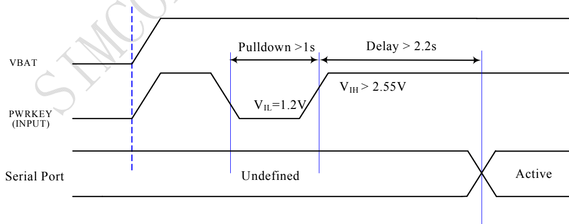
Figure 8: Timing of turn on system using PWRKEY
