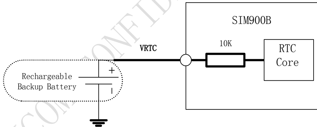
Figure 13: RTC supply from rechargeable battery
