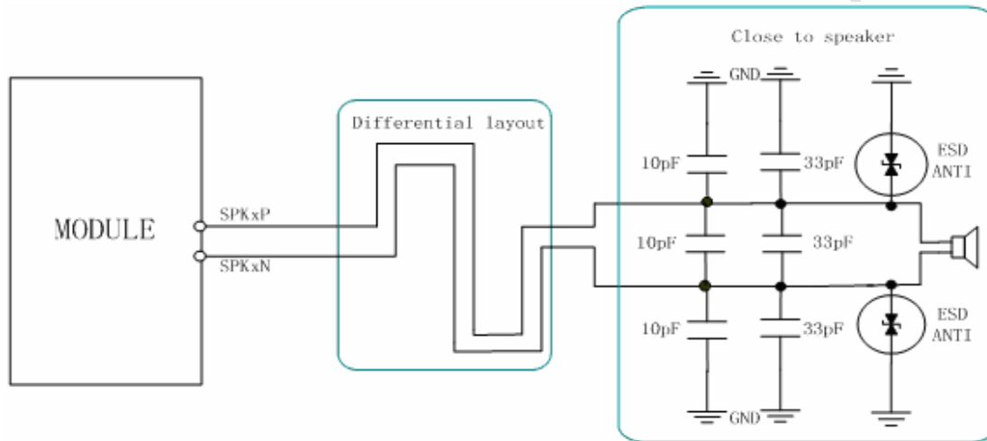
Figure 19: Speaker interface configuration
