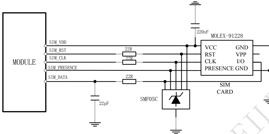
Figure 24: Reference circuit of the 8 pins SIM card
