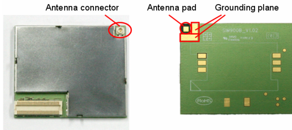
Figure 32 : The RF interface of module
