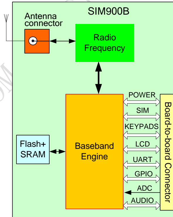
Figure 1: SIM900B functional diagram
