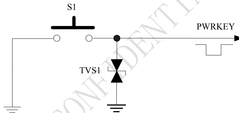
Figure 7: Turn on SIM900B using button
