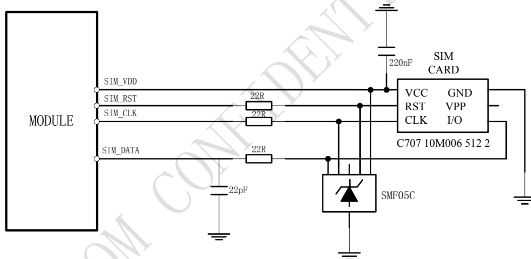
Figure 25: Reference circuit of the 6 pins SIM card
