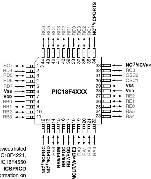
FIGURE 2-2: PIC18F2XX0/2X21/2XX5/4XX0/4X21/4XX5 FAMILY PIN DIAGRAMS
