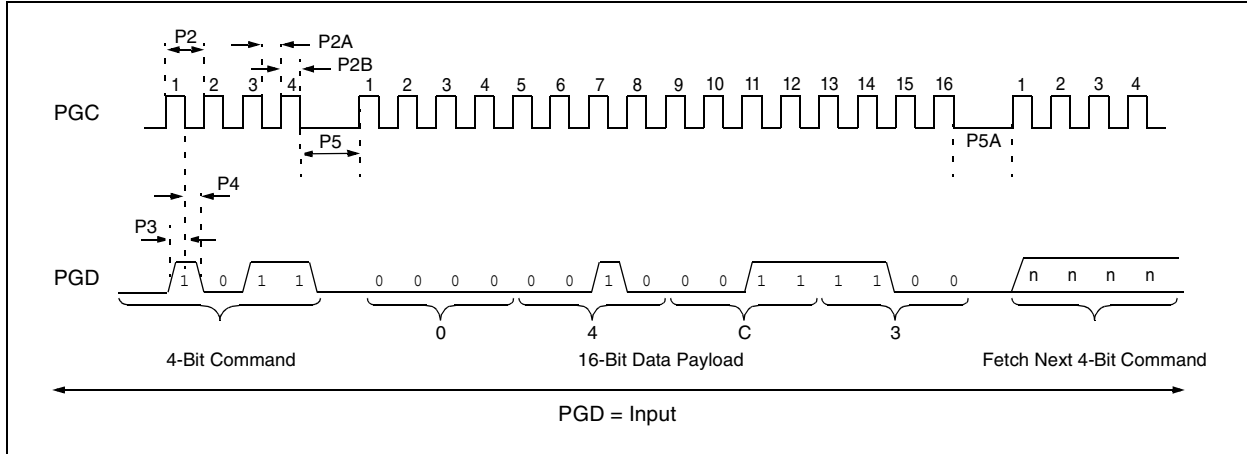
FIGURE 2-14: TABLE WRITE, POST-INCREMENT TIMING (1101)
