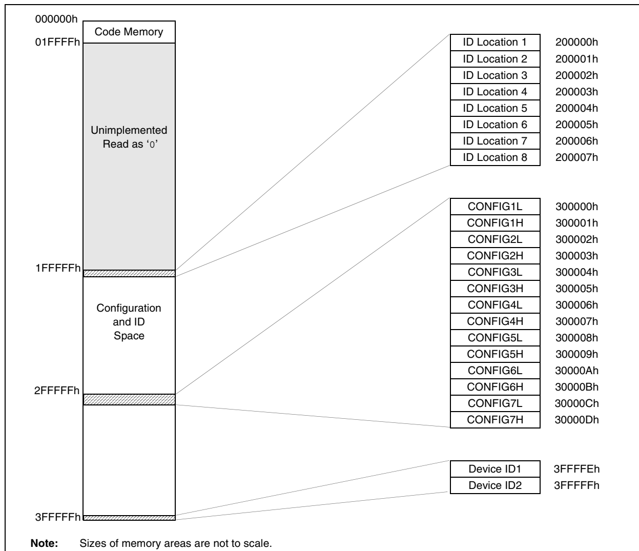
FIGURE 2-8: CONFIGURATION AND ID LOCATIONS FOR PIC18F2XX0/2X21/2XX5/4XX0/4X21/4XX5 DEVICES
