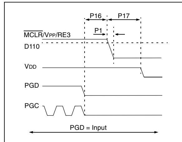
FIGURE 2-11: EXITING HIGH-VOLTAGE PROGRAM/VERIFY MODE
