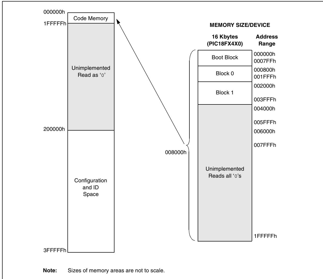
FIGURE 2-5: MEMORY MAP AND THE CODE MEMORY SPACE FOR PIC18FX4X0 DEVICES
