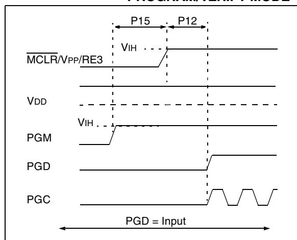
FIGURE 2-12: ENTERING LOW-VOLTAGE PROGRAM/VERIFY MODE
