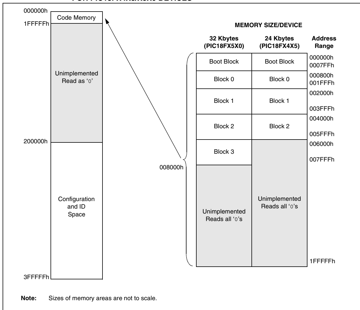
FIGURE 2-4: MEMORY MAP AND THE CODE MEMORY SPACE FOR PIC18FX4X5/X5X0 DEVICES
