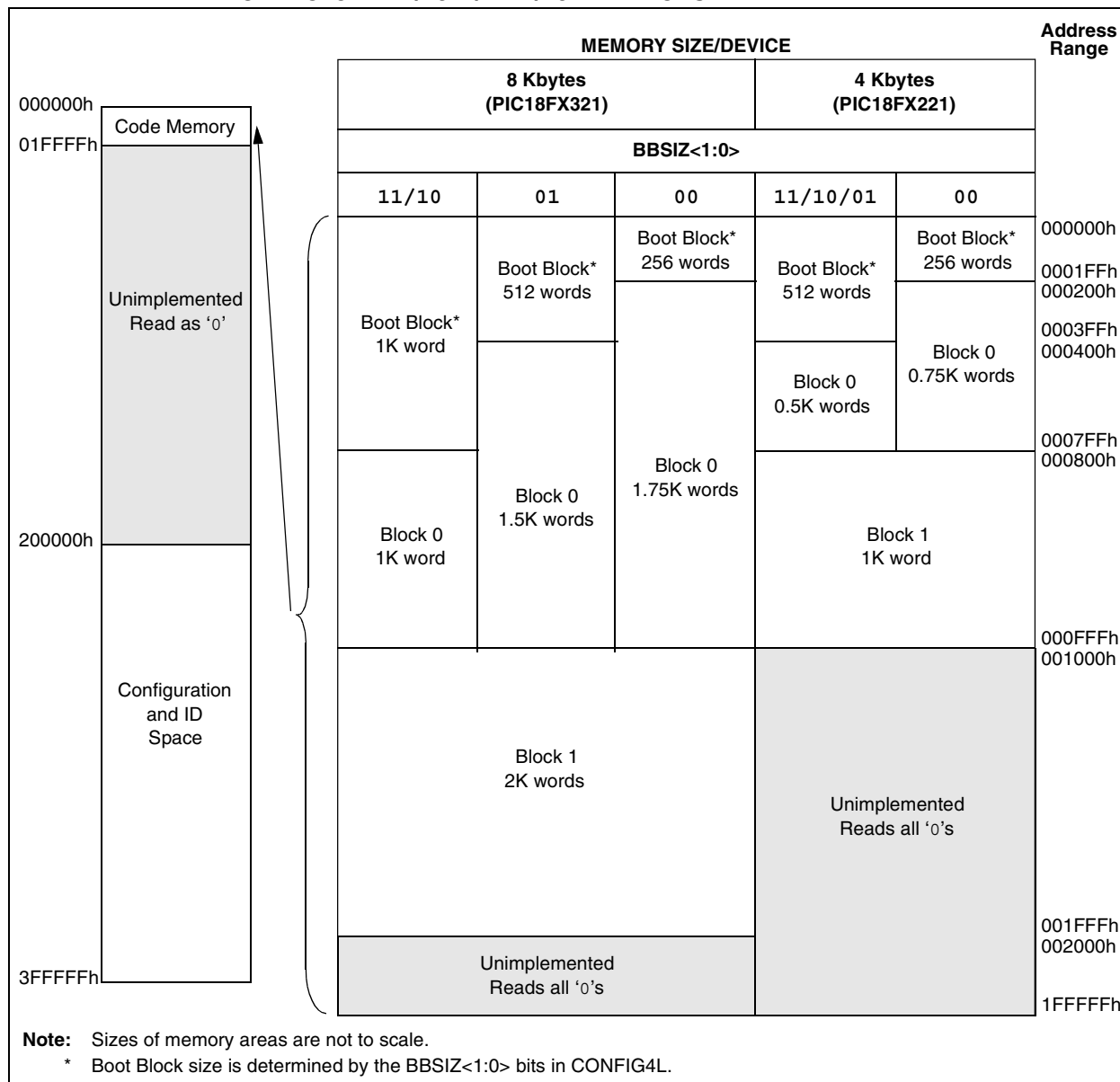
FIGURE 2-7: MEMORY MAP AND THE CODE MEMORY SPACE FOR PIC18F2221/2321/4221/4321 DEVICES
