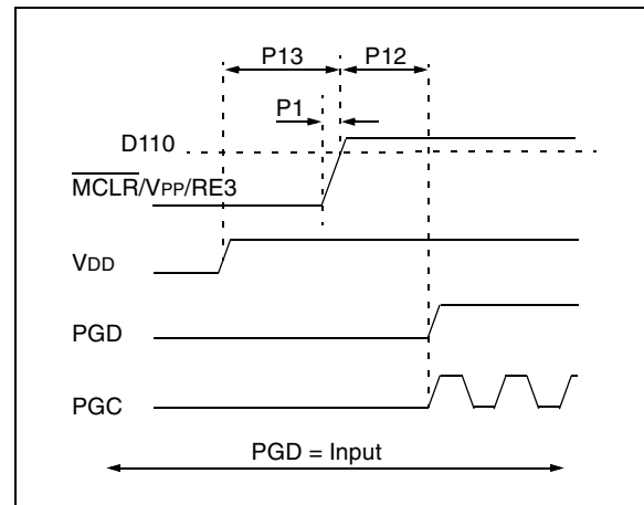
FIGURE 2-10: ENTERING HIGH-VOLTAGE PROGRAM/VERIFY MODE
