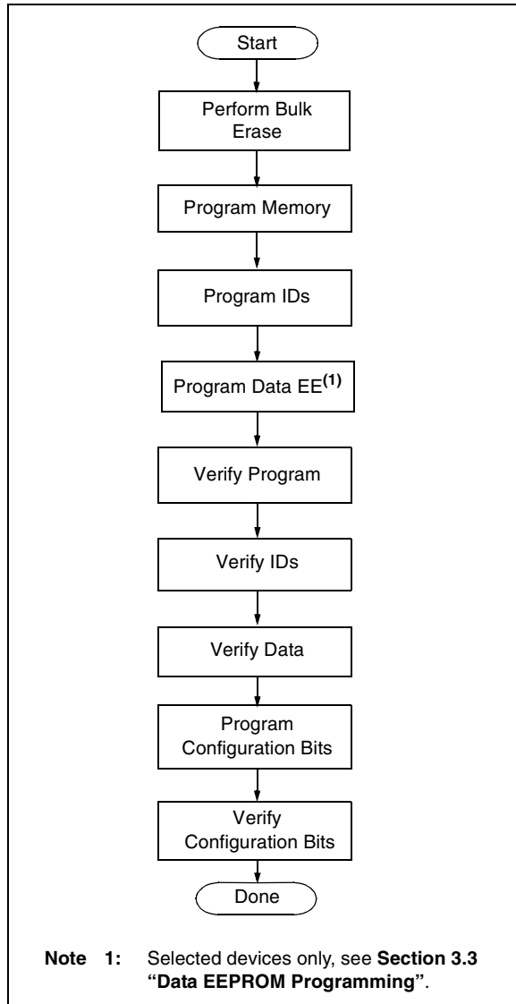
FIGURE 2-9: HIGH-LEVEL PROGRAMMING FLOW
