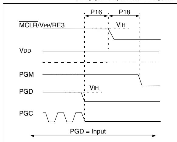
FIGURE 2-13: EXITING LOW-VOLTAGE PROGRAM/VERIFY MODE
