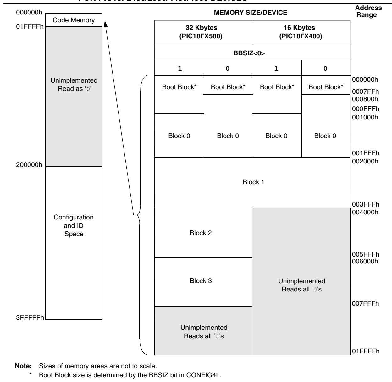
FIGURE 2-6: MEMORY MAP AND THE CODE MEMORY SPACE FOR PIC18F2480/2580/4480/4580 DEVICES
