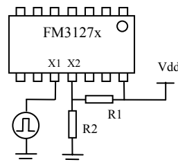
Figure 8. External Oscillator
