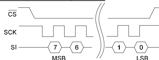
Figure 12. SPI Modes 0 & 3
