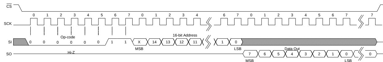
Figure 20. Memory Read
