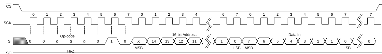
Figure 19. Memory Write
