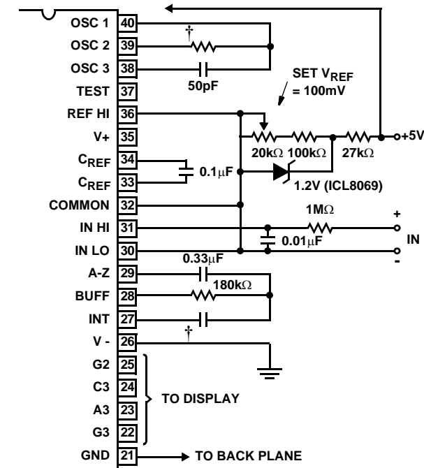
FIGURE 14. ICL7126 OPERATED FROM SINGLE +5V SUPPLY An external reference must be used in this application, since the voltage between V+ and V- is insufficient for correct operation of the internal reference. † indicates values depend on clock frequency.
