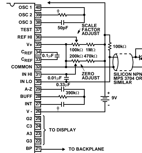
FIGURE 16. ICL7126 USED AS A DIGITAL CENTIGRADE THERMOMETER A silicon diode-connected transistor has a temperature coefficient of about -2mV/°C. Calibration is achieved by placing the sensing transistor in ice water and adjusting the zeroing potentiometer for a 000.0 reading. The sensor should then be placed in boiling water and the scale-factor potentiometer adjusted for a 100.0 reading.
