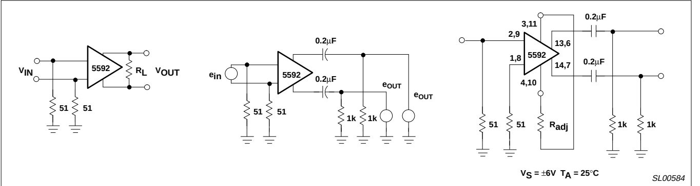
Figure 3. Test Circuits
