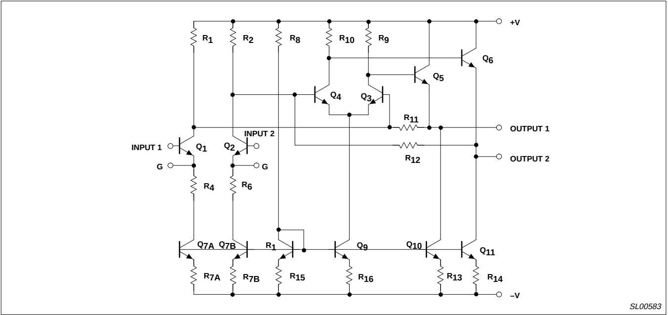
Figure 2. Equivalent Circuit
