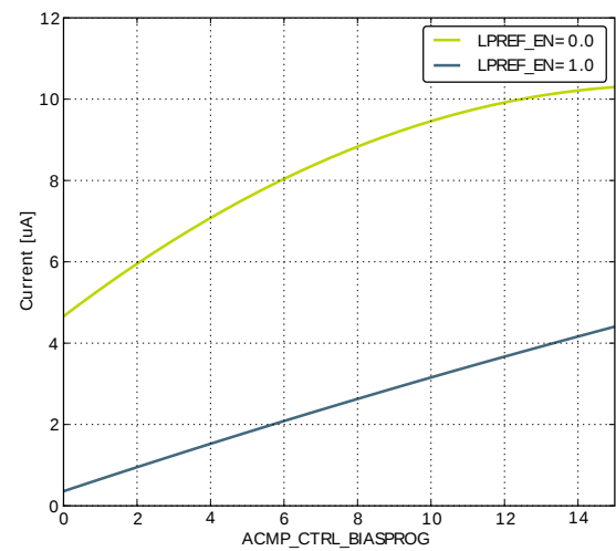
Current consumption
