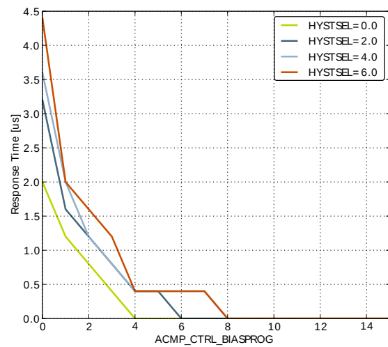
Response time
