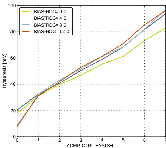
Hysteresis
