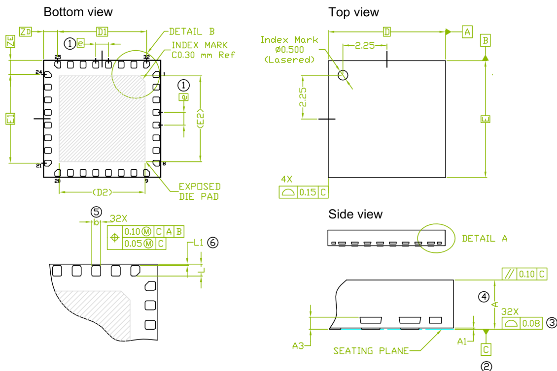
Figure 4.2. QFN32
