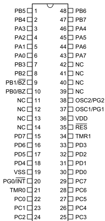
HT48R50A-1 - 48 SSOP-A
