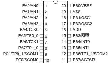
HT66F14 20 DIP-A/SOP-A/SSOP-A
