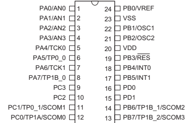
HT66F15 24 SKDIP-A/SOP-A/SSOP-A
