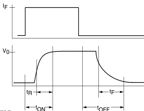
Fig. 2 Switching Waveform
