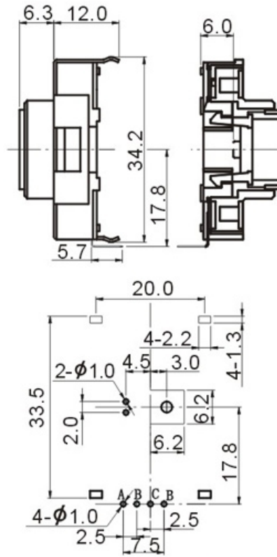
P.C.B. MOUNTING DETAIL
